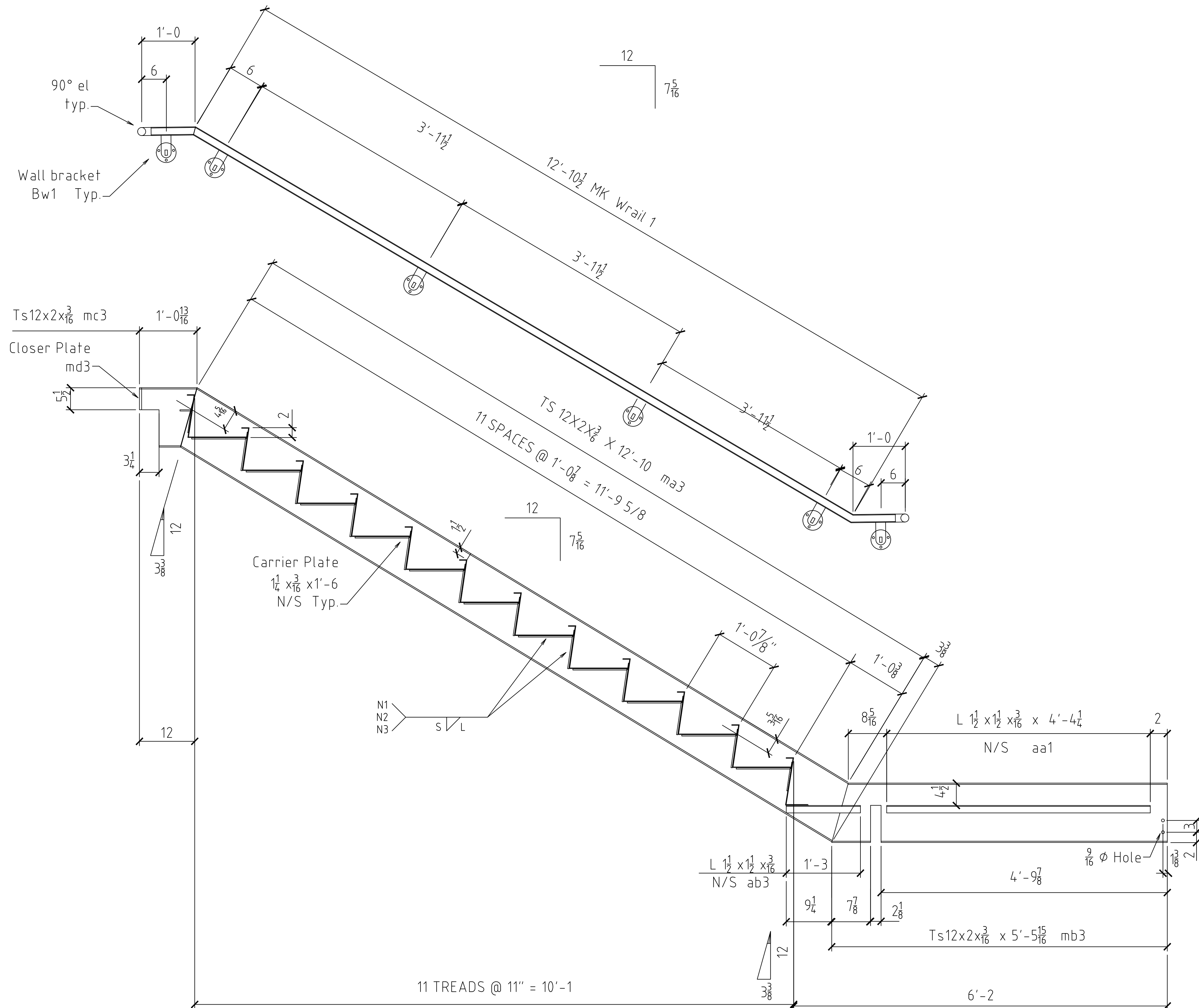
STRINGER ASSEMBLY MK ST3 From 6'-8" Elv. to 13'-4" From 20'-0" Elv. to 26'-8"
